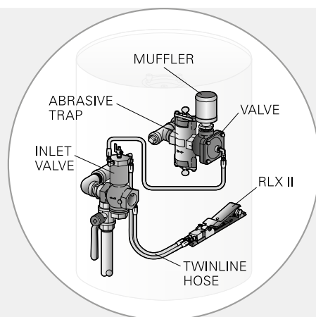
AX Quick Acting Electric Deadman Remote Control
