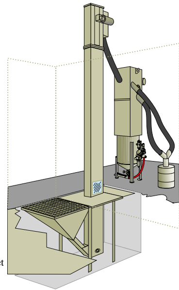
3 X 3 HOPPER SYSTEM
