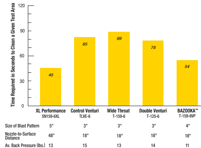
Figure 2. Nozzle Performance Comparison
