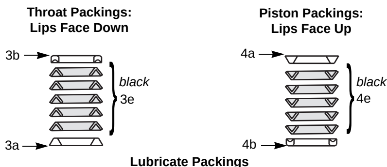
FIG. 6: Tuff-Stack™ Seals Repair Kits
